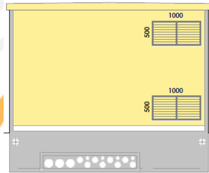
FAÇADE ARRIERE
